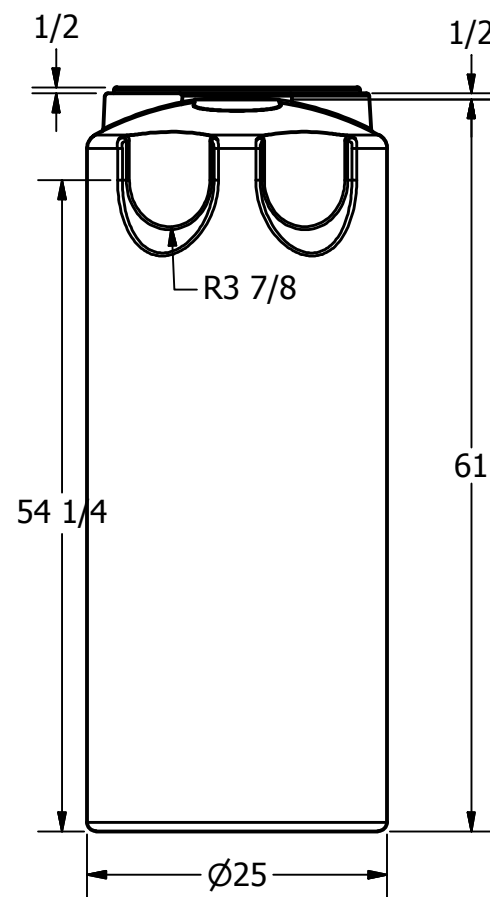
SECTION A-A SCALE 1 / 16
