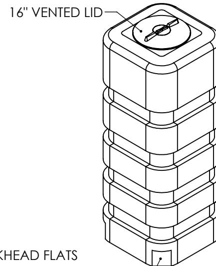
ISOMETRIC VIEWS
