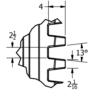
DETAIL C SCALE 1 / 11
